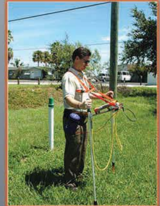
PIPELINE SURVEYS
